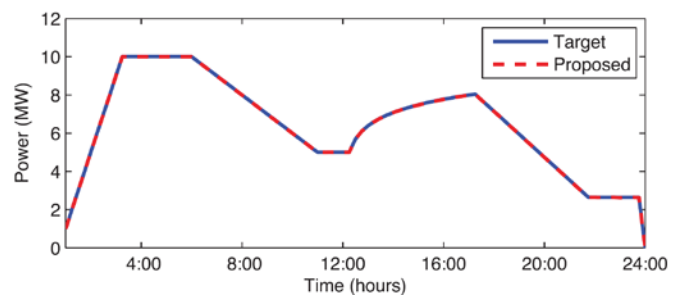
Figure 71: Power tracking of 20000 EVs with heterogenous plugging time (Malhotra et al., 2017)
