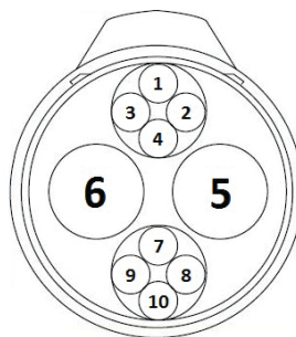
Figure 10: ChaDeMo DC charging connector
