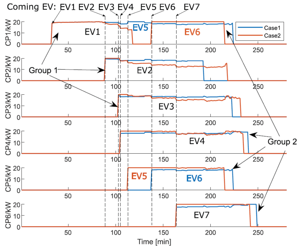
Figure 88: Charging coordination comparison (Yan et al., 2021)
