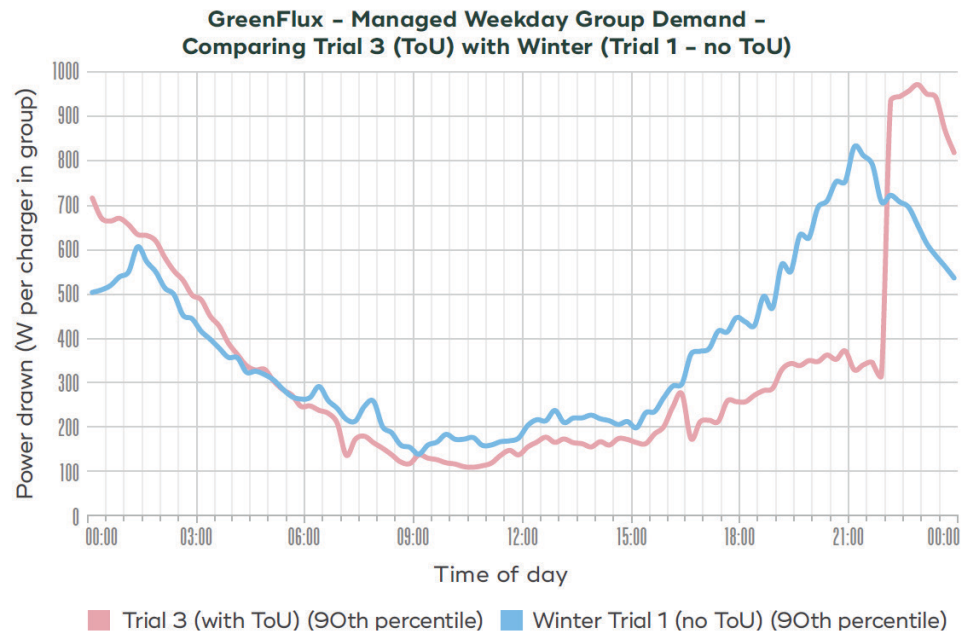
Figure 46: Charging behaviour without and with incentivisation ("Powered-Up-Electric-Nation-Brochure.pdf," n.d.)
