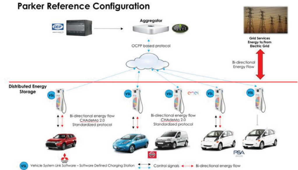
Figure 47: System configuration in Parker project ("Parker_Final-report_v1.1_2019.pdf," n.d.)
