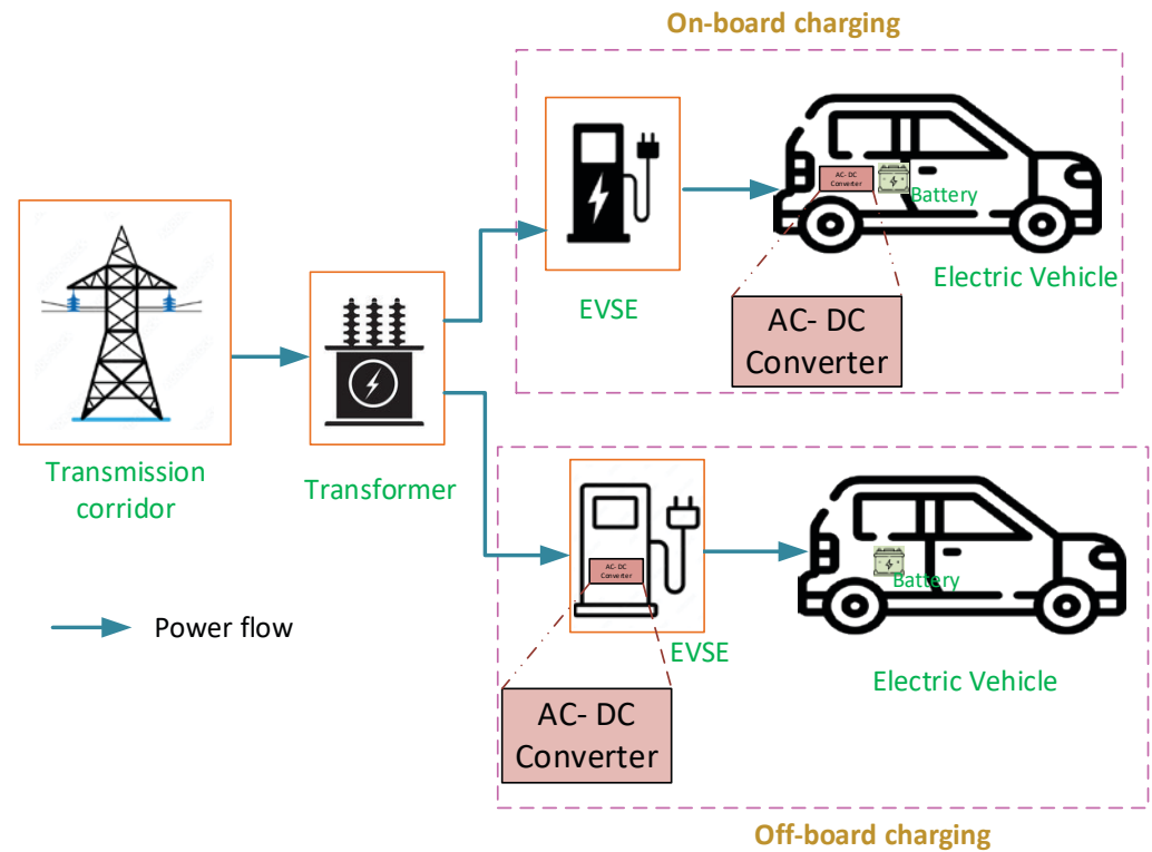
Figure 3 : AC and DC conductive charging ecosystem
