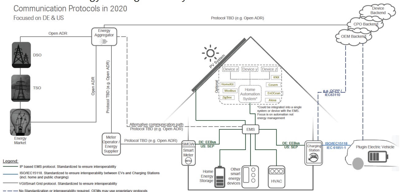
Figure 14: Example for communication infrastructure in private households with possible communication protocols for different applications (Verband der Automobilindustrie 2020)
