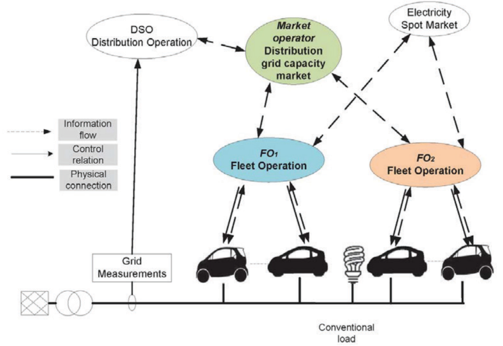
Figure 61: Network architecture of low voltage distribution system (Hu et al., 2014)
