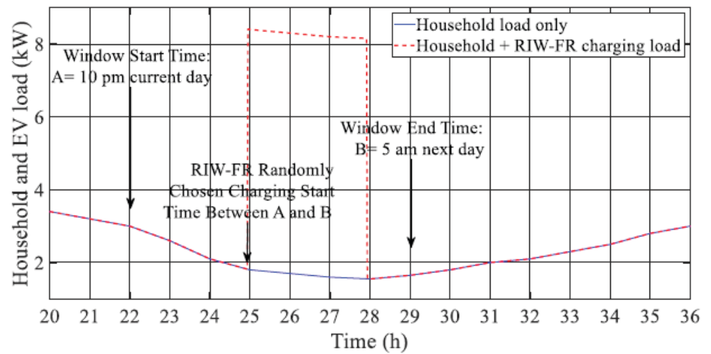
Figure 79: RIW charging profile of one EV load (Mobarak and Bauman, 2019)
