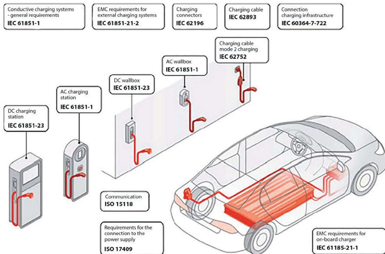
Figure 13: Wired charging and related standards of EVs (Nationale Plattform Elektromobilität)
